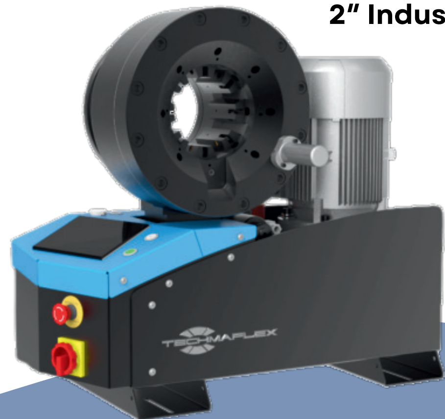
Crimping Machine Techmaflex S-Crimp 350 EVO 3" 2WB 2" 4WS & 6WS 4" Textile/Suction Hose
