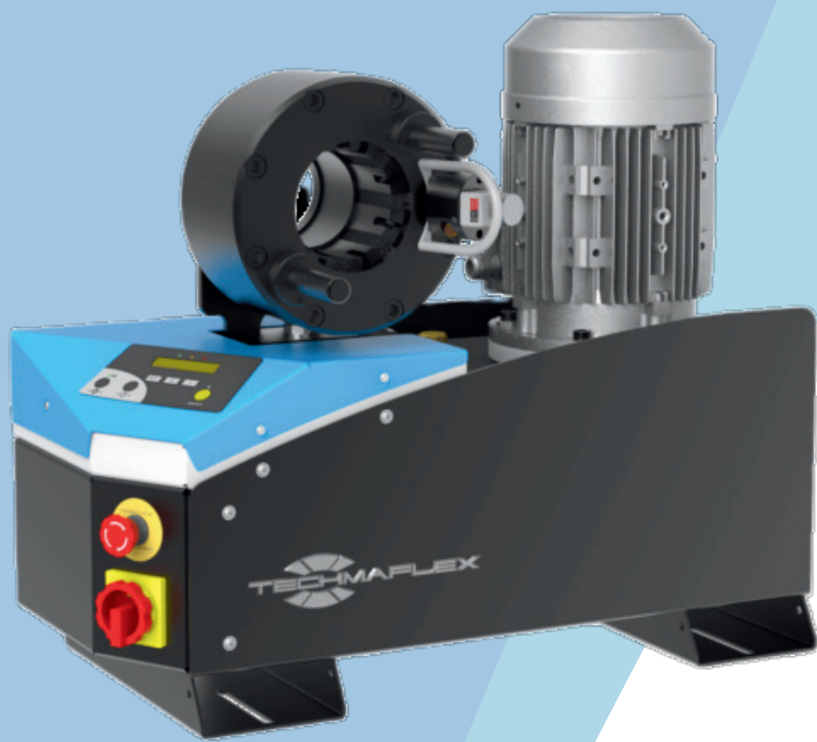
Crimping Machine Techmaflex S-Crimp 137 EVO 1"-1/4 2WB & 4WS 1"-1/2 Industrial
